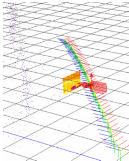
Figure 6: Camera path and point cloud of corresponding points of the image sequence
