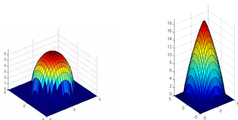
Figure 2: 3D visualisation of the Pollock-Model. Left: Surface model of a typical deciduous tree: a=7 , b=3.5 , n=2.0 Right: Coniferous tree: a=20.0 ; b=5.0 ; n=1.2 .
