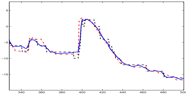
Figure 5: Synthetic data: profiles of the true height map (red and dash-dotted), the L1-norm regularized map (black and dashed) and refined L2-L1 estimation (plain blue) — \lambda = 1.5 and 50 steps of projected gradient descent
